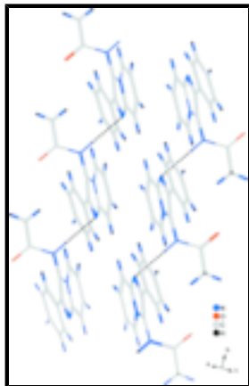
Fig. 3. The columns of molecules showing N—H...N hydrogen bonds
