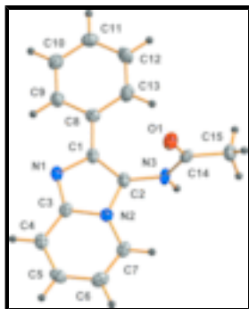
Fig. 2. Asymmetric unit of title compound, showing 50% displacement ellipsoids for non-H atoms.
